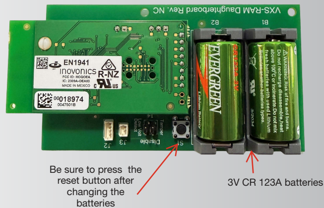
Fig. 1 (transmitter with case open)
